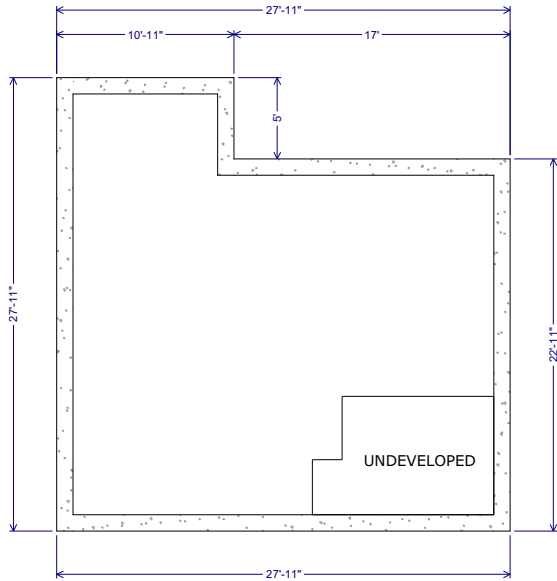
BASEMENT
