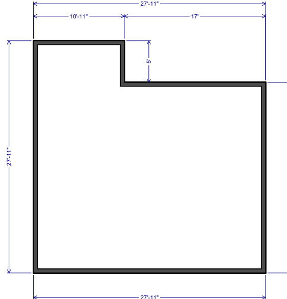
MAIN LEVEL
